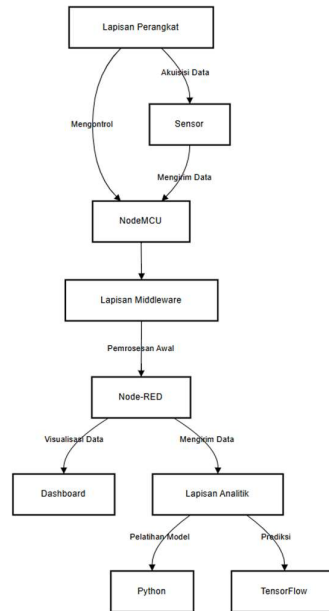
GAMBAR 1: Diagram Blok Arsitektur Sistem Smart Building
