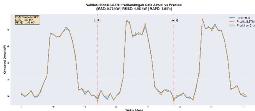
GAMBAR 7: Validasi Model - Perbandingan Data Aktual vs Prediksi LSTM
